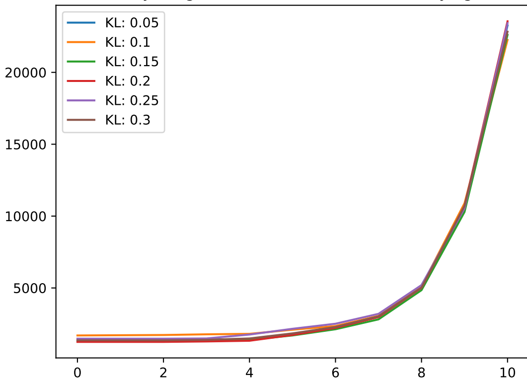
Memory usage of SVM for moon data of varying KL
